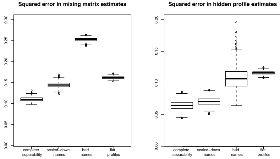
FIG 3. Total mean squared error across all elements of the mixing matrix and latent profile matrix. The vertical axis is the sum of the errors across all eight alter groups. We generated 500 respondents using the four profile structures then evaluated our ability to recover the mixing matrix estimated in McCormick et al. (2010) and the known profiles of six additional names. We repeated the simulation 1,000 times. In both cases the ideal profile has the lowest error, followed by the scaled-down names suggested by McCormick et al. (2010) .
