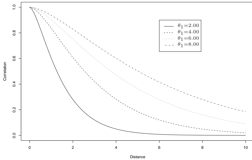
Figure 2: Matern autocorrelation function for smoothness parameter \theta_2 = 1.00 and various range parameter values, \theta_1 .
