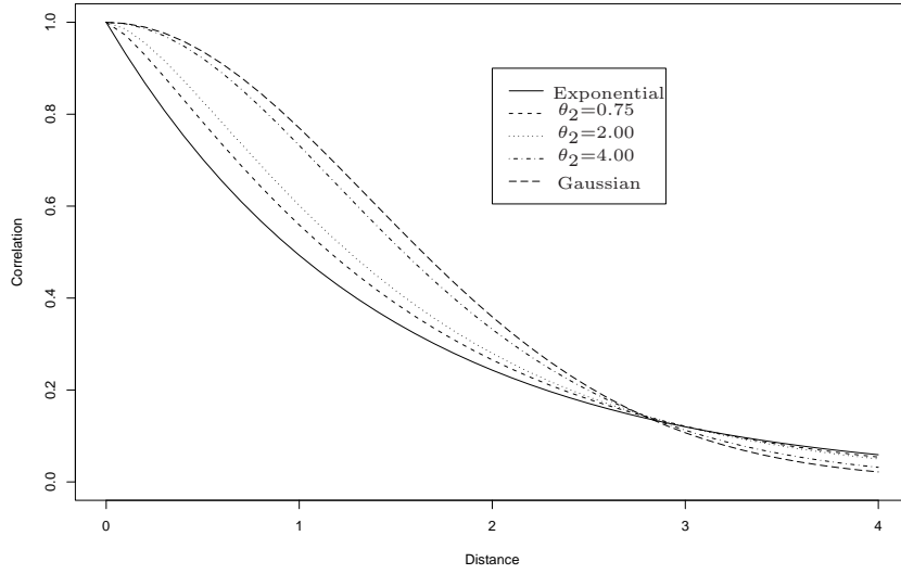
Figure 1: Matern autocorrelation function for several parameter values. The horizontal axis is the distance between points and the vertical axis is the correlation between two points at a given distance. We used a fixed range parameter, \theta_1 = 2.00 , with various smoothness parameter values, \theta_2 . Note that the exponential autocorrelation is equivalent to the Matern autocorrelation function with \theta_2 = 0.50 and that the Gaussian autocorrelation function corresponds to the limiting case such that \theta_2 \rightarrow \infty .
