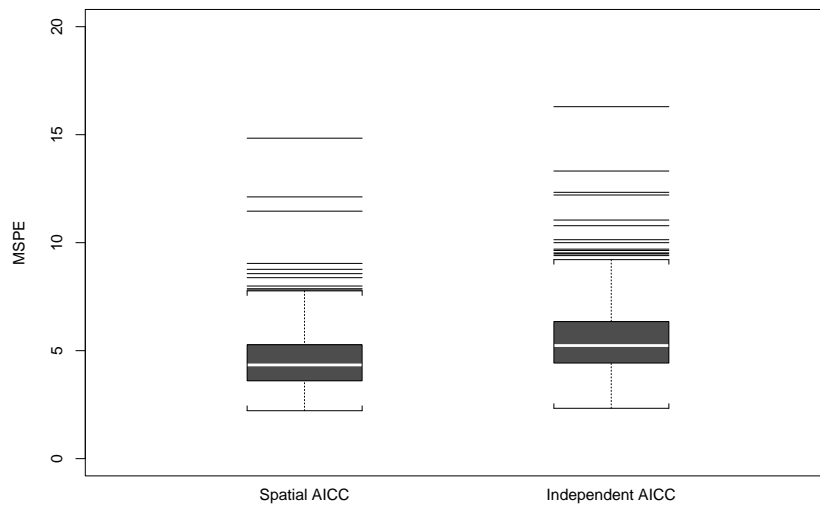
Figure 5: Mean Squared Prediction Error (MSPE) for the two model selection methods based on 500 simulations.
