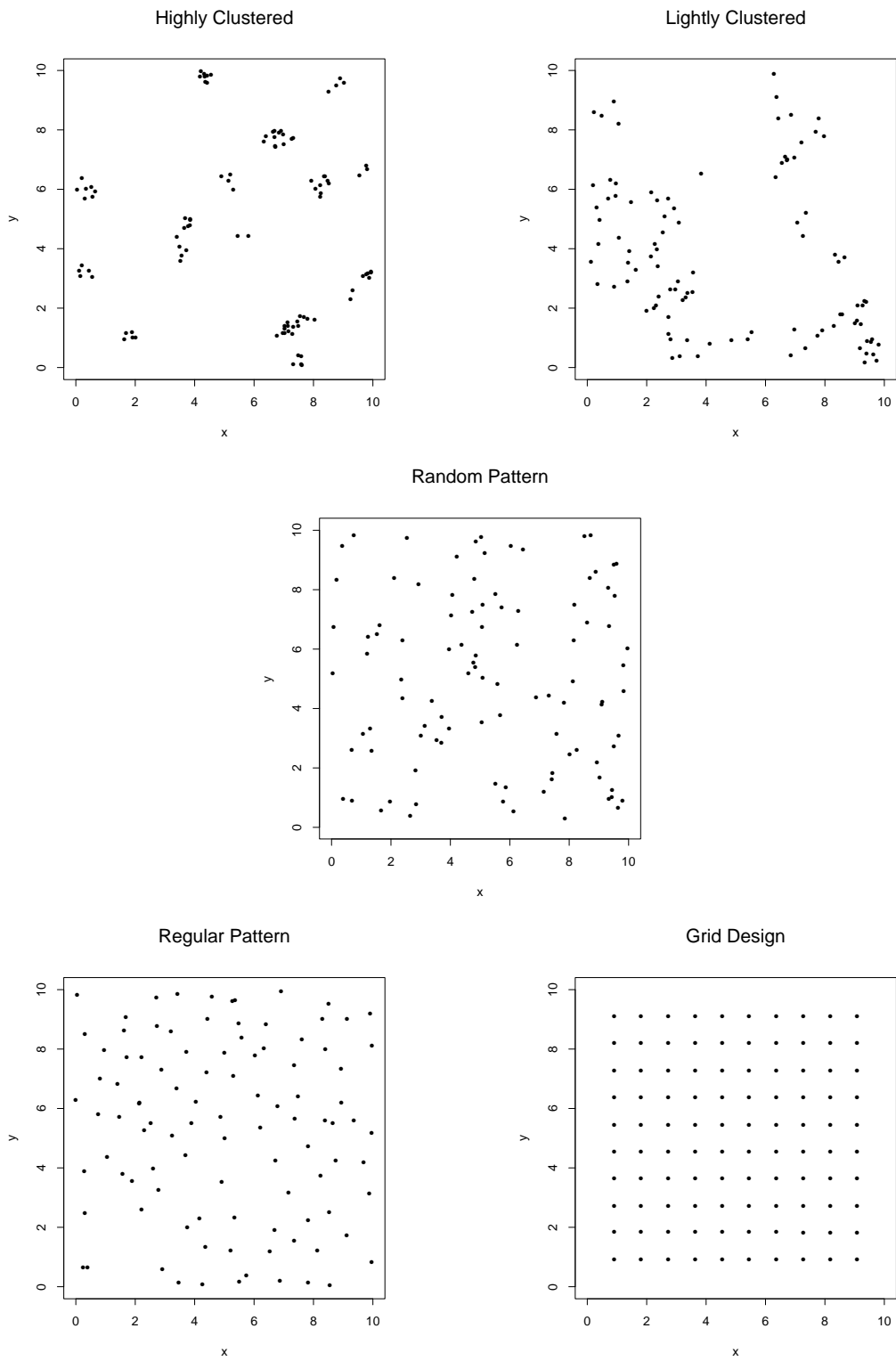
Figure 4: Five Sampling Patterns
