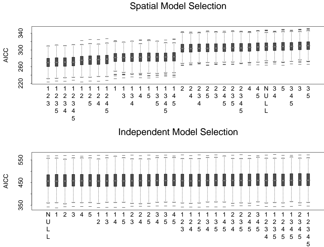
Figure 3: AICC values for the spatial AICC and independent AICC selection strategies. Note that the models for the spatial AICC method have been ordered from smallest to largest average AICC over all 500 simulations. The horizontal axis lists the variables included in each model where NULL refers to the intercept-only model.
