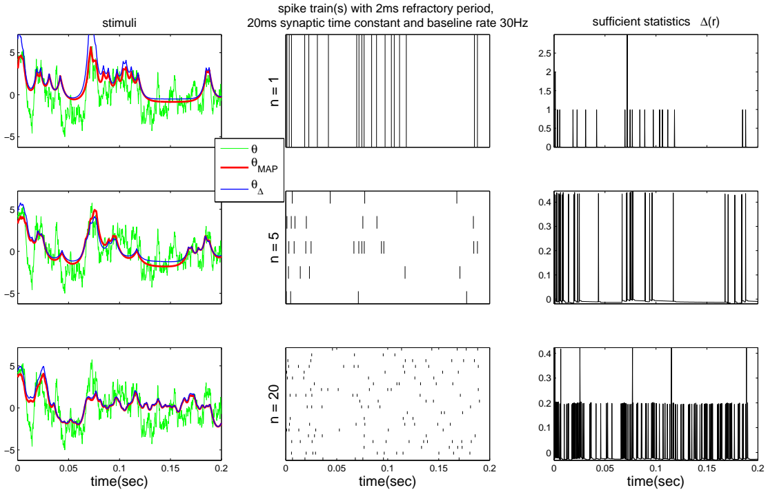
Figure 1: The left panels show the true stimulus (green), MAP estimate (red) and the limiting optimal estimator \hat{\theta}_{\Delta} := (J + C_{\theta}^{-1})^{-1}\Delta(r) (blue) for various population sizes n . The middle panels show the spike trains used to compute these estimates. The right panels show the sufficient statistics \Delta(r) used to compute \hat{\theta}_{\Delta} . Note that the same true stimulus was used in all three simulations. As n increases, the linear decoder converges to the MAP estimate, despite the nonlinear and correlated nature of the network model generating the spike trains (see main text for details).
