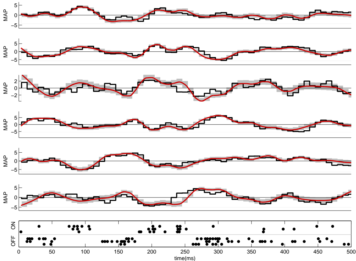
Figure 5: MAP decoding of the spatio-temporal stimulus \mathbf{k}_i * x(t) from the simultaneously recorded spike trains of three pairs of ON and OFF retinal ganglion cells, again from [77]. The top six panels show the true input \mathbf{k}_i * x(t) to each cell (jagged black line; the filters \mathbf{k}_i were estimated by maximum likelihood from a distinct training set here), and the decoded MAP estimate (smooth curve) \pm 1 posterior s.d. (gray area). The MAP estimate is quite accurate and is computed in O(T) time, where T is the stimulus duration. In this example, fully-Bayesian Markov chain Monte Carlo decoding produced nearly identical results; see [1] for details.
