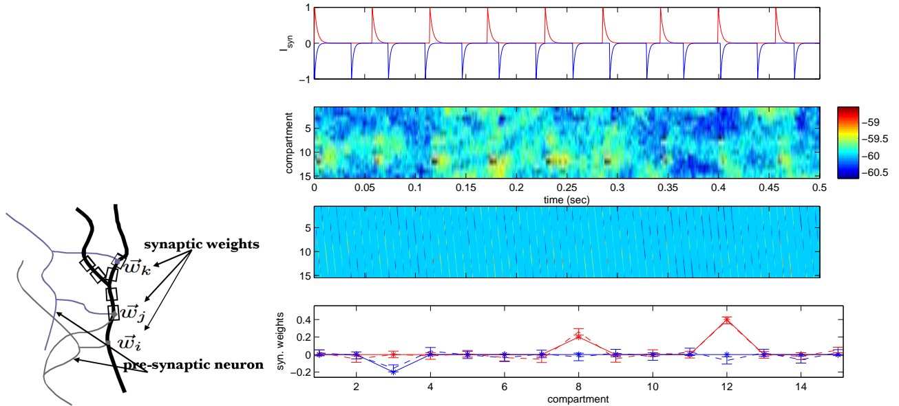
Figure 4: Estimating the location and strength of synapses on a simulated dendritic branch. Left: simulation schematic. By observing a noisy, subsampled spatiotemporal voltage signal on the dendritic tree, we can infer the strength of a given presynaptic cell’s inputs at each location on the postsynaptic cell’s dendritic tree. Right: illustration of the method applied to simulated data [73]. We simulated two presynaptic inputs: one excitatory (red) and one inhibitory (blue). The (known) presynaptic spike trains are illustrated in the top panel, convolved with exponential filters of \tau = 3 ms (excitatory) and \tau = 2 ms (inhibitory) to form U_t . Second panel: True (unobserved) voltage (mV), generated from the cable equation (13). Note that each presynaptic spike leads to a post-synaptic potential of rather small magnitude (at most \approx 1 mV), relative to the voltage noise level. In this case the excitatory presynaptic neuron synapses twice on the neuron, on compartment 12 and a smaller synapse on compartment 8, while the inhibitory neuron synapses on compartment 3. Third panel: Observed (raster-scanned) voltage. The true voltage was not observed directly; instead, we only observed a noisy, spatially-rastered (linescanned), subsampled version of this signal. Note the very low effective SNR here. Bottom panel: True and inferred synaptic weights. The true weight of each synapse is indicated by an asterisk (*) and the errorbar shows the posterior mean E(\theta_i|Y) and standard deviation \sqrt{Var(\theta_i|Y)} of the synaptic weight given the observed data. Note that inference is quite accurate, despite the noisiness and the brief duration (500 ms) of the data.
