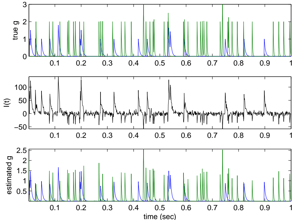
Figure 3: Inferring presynaptic inputs given simulated postsynaptic voltage recordings. Top: true simulated conductance input (green indicates inhibitory conductance; blue excitatory). Middle: observed noisy current trace from which we will attempt to infer the input conductance. Bottom: Conductance inferred by nonnegative MAP technique. Note that inferred conductance is shrunk in magnitude compared to true conductance, due to the effects of the prior p(N_t^E) and p(N_t^I) , both of which peak at zero here; shrinkage is more evident in the inferred inhibitory conductance, due to the smaller driving force (the holding potential in this experiment was -62 mV, which is quite close to the inhibitory reversal potential; as a result, the likelihood term is much weaker for the inhibitory conductance than for the excitatory term). Inference here required about one second on a laptop computer per second of data (i.e., real time), at a sampling rate of 1 KHz.
