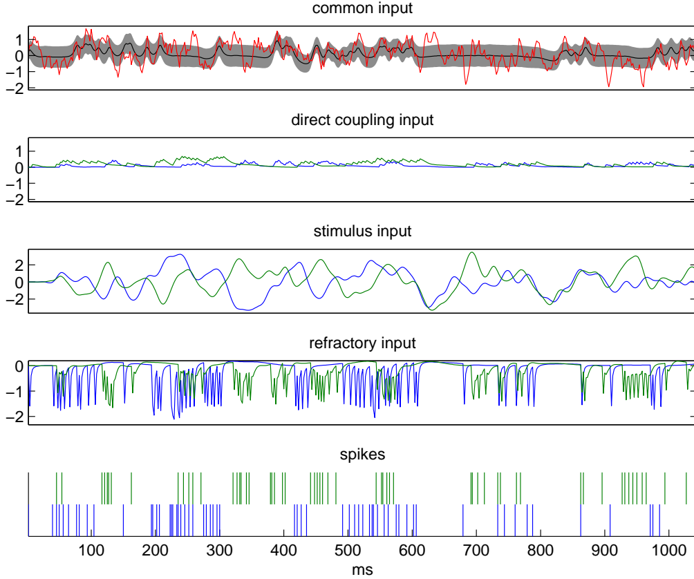
Figure 2: Single-trial inference of the relative contribution of common, stimulus, direct coupling, and self inputs in a pair of retinal ganglion ON cells [104]; data from [77]. Top panel: Inferred linear common input, \hat{Q} : red trace shows a sample from the posterior distribution p(Q|Y) , black trace shows the conditional expectation E(Q|Y) , and shaded region indicates \pm 1 posterior standard deviation about E(Q|Y) , computed from the diagonal of the inverse log-posterior Hessian H . 2^{nd} panel: Direct coupling input from the other cell, \mathbf{l}_j \cdot \mathbf{y}_j . (The first two panels are plotted on the same scale to facilitate comparison of the magnitudes of these effects.) Blue trace indicates cell 1; green indicates cell 2. 3^{rd} panel: The stimulus input, \mathbf{k} \cdot \mathbf{x} . 4^{th} panel: Refractory input, \mathbf{h}_i \cdot \mathbf{y}_i . Note that this term is strong but quite short-lived following each spike. All units are in log-firing rate, as in equation (7). Bottom: Observed paired spike trains Y on this single trial. Note the large magnitude of the estimated common input term \hat{q}(t) , relative to the direct coupling contribution \mathbf{l}_j \cdot \mathbf{y}_j .
