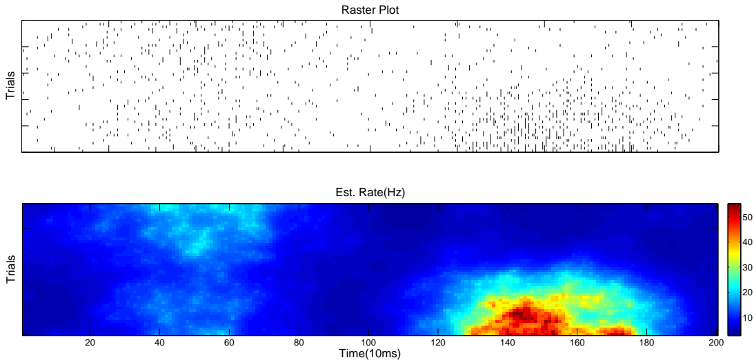
Figure 6: An example of the fast spatial estimation method applied to data from [17], Fig. 3. Top panel: observed spike train data. Note that the firing rate qualitatively changes both as a function of time t and trial number i ; 50 trials total are observed here. Bottom: \lambda(t, i) estimated using the fast regularized methods described in [81]. See [81] for further comparisons, e.g. to linear kernel smoothing methods.
