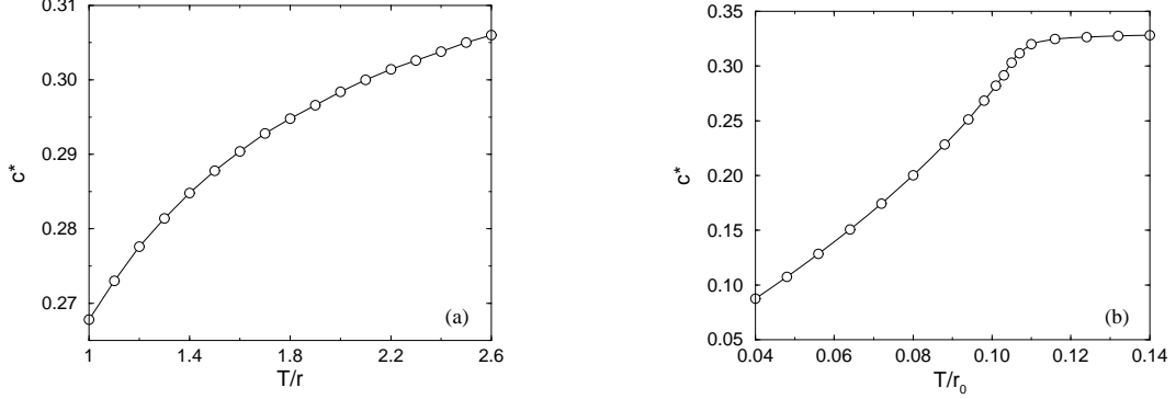
FIG. 3: Simulation results for the fixed point minority concentration c^* for: (a) a population of N = 5000 agents with constant strategic bias as a function of x = \frac{T}{r} , and (b) N = 50000 agents with state-dependent strategic bias as a function of x_0 = \frac{T}{r_0} . The numerical value c^* , which agrees perfectly with the rate equation predictions, is determined by the time integral of the concentration divided by the observation time. The change in behavior when x_0 \approx \frac{1}{9} becomes a cusp as N \rightarrow \infty .
