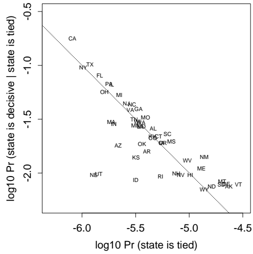
Figure 3: Probability that state is decisive given tied vs. probability the state is tied for 1992 plotted on log scale. The dotted line corresponds to a product of 10^{-7} .
