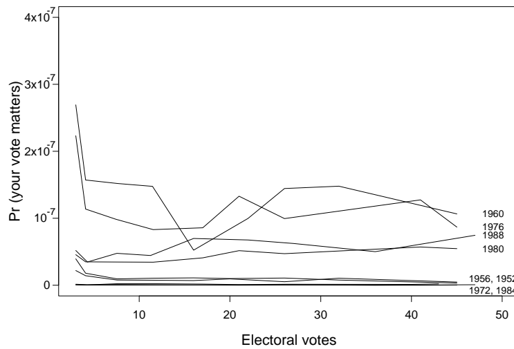
Figure 2: Same plot as in Figure 1 for model with \theta set to 1 (that is, state-level variance inversely proportional to turnout).
