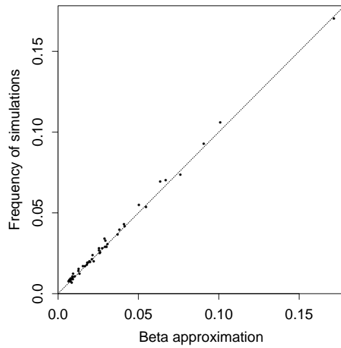
Figure 4: Estimated probability that state is decisive given tied, computed based on frequency of simulations vs. estimate from fitted beta distribution. The dotted line corresponds to equality of probabilities.
