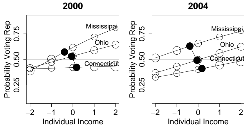
Figure 4: From the multilevel logistic regression model with varying intercepts and slopes fit to Annenberg poll data from 2000 and 2004: probability of supporting Bush as a function of income category, for a rich state (Connecticut), a middle-income state (Ohio), and a poor state (Mississippi). The open circles show the relative proportion (as compared to national averages) of households in each income category in each of the three states, and the solid circles show the average income level and estimated average support for Bush for each state. Income is a very strong predictor of vote preference in Mississippi, a weaker predictor in Ohio, and only weakly predicts vote choice at all in Connecticut. See Figure 5 for estimated slopes in all 50 states, and compare to Figure 3, in which the state slopes are constrained to be equal.
