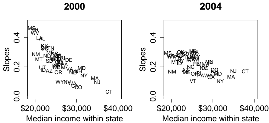
Figure 5: Estimated coefficients for income within state plotted vs. average state income, for the varying-intercept, varying-slope multilevel model fit to the Annenberg survey data from 2000 and 2004.
