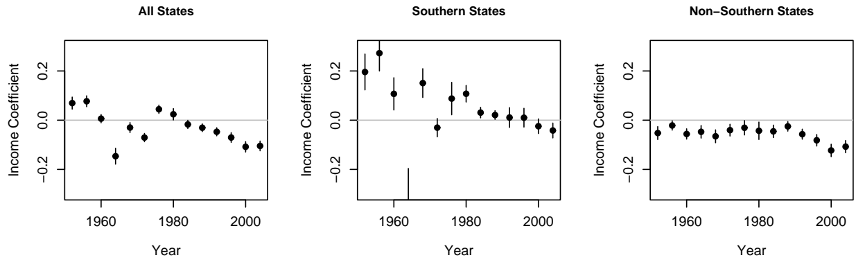
Figure 1: (a) Coefficients for average state income (in tens of thousands of 1996 dollars) in regressions predicting Republican vote share by state. The model was fit separately for each election year. Estimates and standard errors are shown. (b, c) Same model but fit separately to Southern and non-Southern states each year. In recent years, Republicans have done better in poor states than in rich states.
