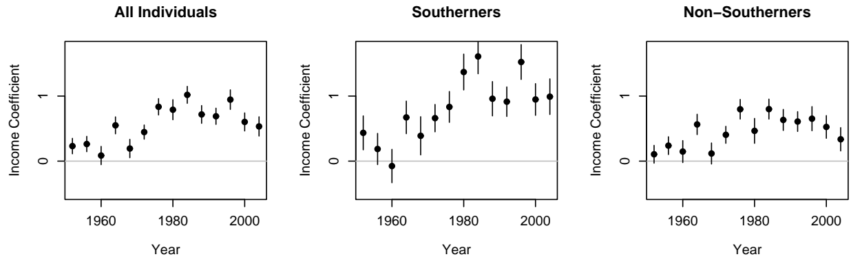
Figure 2: Coefficients and standard errors for income in logistic regressions of Republican vote, fit to NES data from each year. The positive coefficients indicate that higher-income voters have consistently supported the Republicans, a pattern that holds both within and outside the South.
