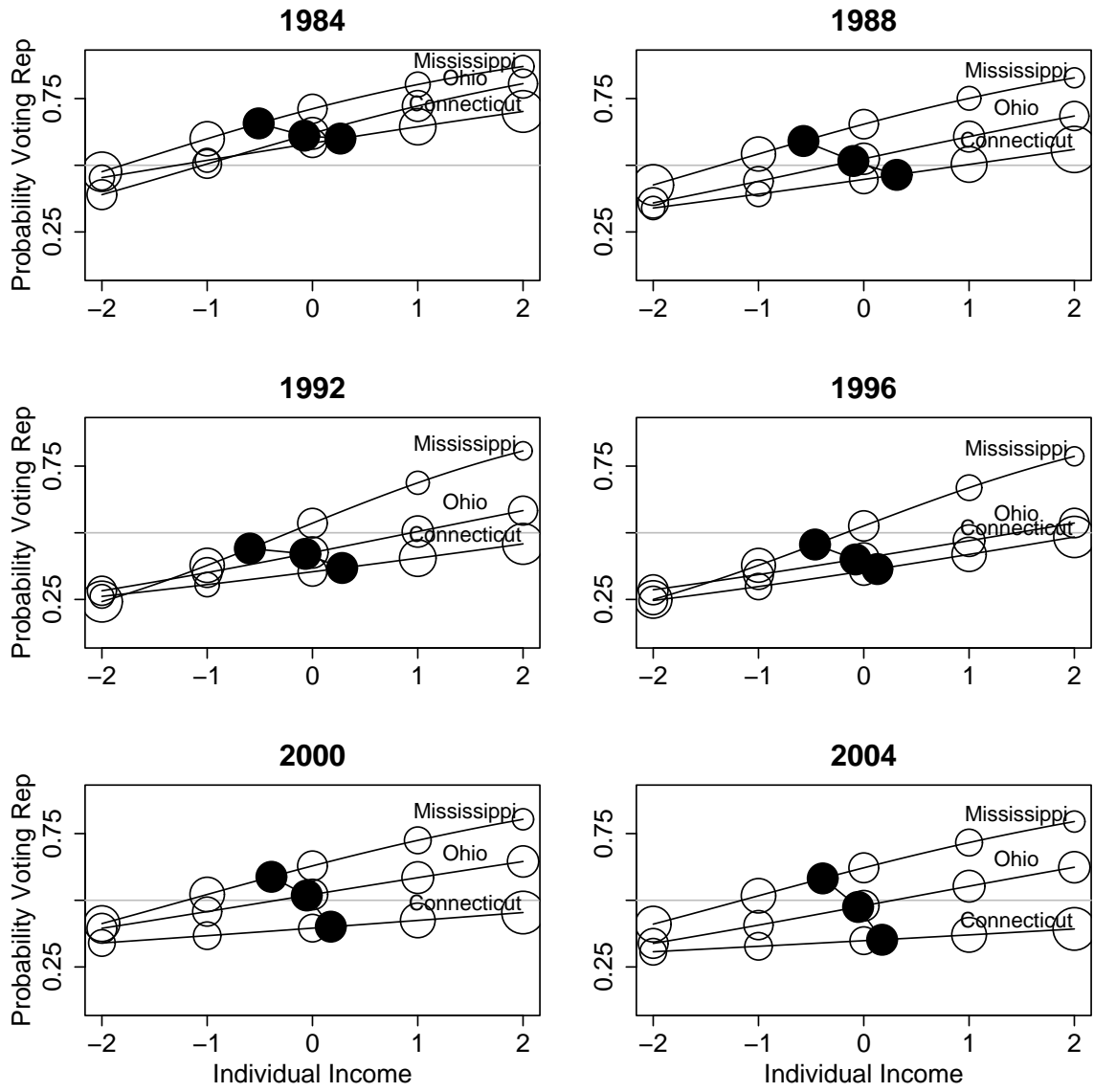
Figure 6: Using exit poll data from 1984–2004, results for the varying-intercept, varying-slope multilevel logistic regression. The curves show the probability of supporting Bush as a function of income category, within states that are poor, middle-income, and rich.
