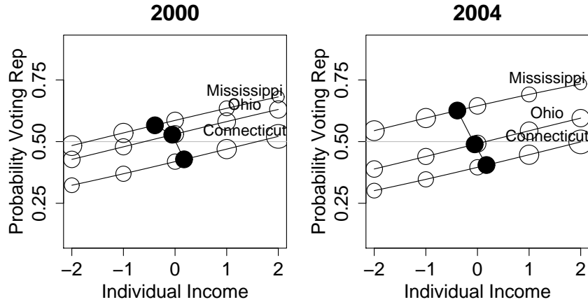
Figure 3: The paradox is no paradox. From the varying-intercept multilevel logistic regression model fit to Annenberg poll data from 2000 and 2004: probability of supporting Bush as a function of income category, for a rich state (Connecticut), a middle-income state (Ohio), and a poor state (Mississippi). The open circles show the relative proportion (as compared to national averages) of households in each income category in each of the three states, and the solid circles show the average income level and estimated average support for Bush for each state. Within each state, richer people are more likely to vote Republican, but the states with higher income give more support to the Democrats.
