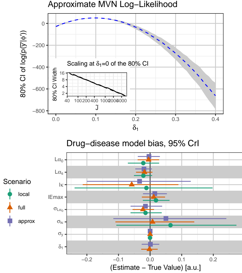
FIG 3. Drug-disease model example: (Top) Assessment of the distribution of the multivariate normal approximation to \log p(\bar{y}|\phi') at a simulation size of \tilde{J} = 10^2 hypothetical fake patients using 10^3 replicates for varying \delta_1 . The gray area marks the 80% confidence interval, the blue dotted line is the median of the simulations. The inset shows the width of the 80% confidence interval at \delta_1 = 0 as a function of the simulation size \tilde{J} on a log-log scale. The dotted line has a fixed slope of -1/2 and the intercept was estimated using least squares. (Bottom) The model estimates are shown as bias for the three different scenarios as discussed in the text. Lines show the 95% credible intervals of the bias and the center point marks the median bias. The MCMC standard error of the mean is for all quantities below 10^{-3} .
