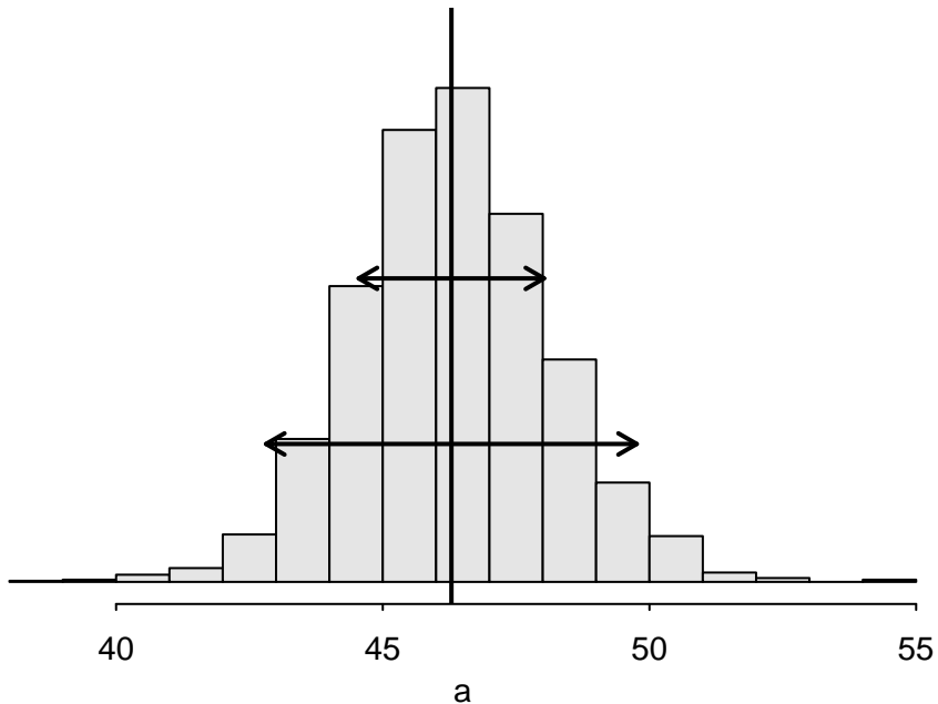
Posterior simulations of the intercept, a , and posterior median \pm 1 and 2 std err
