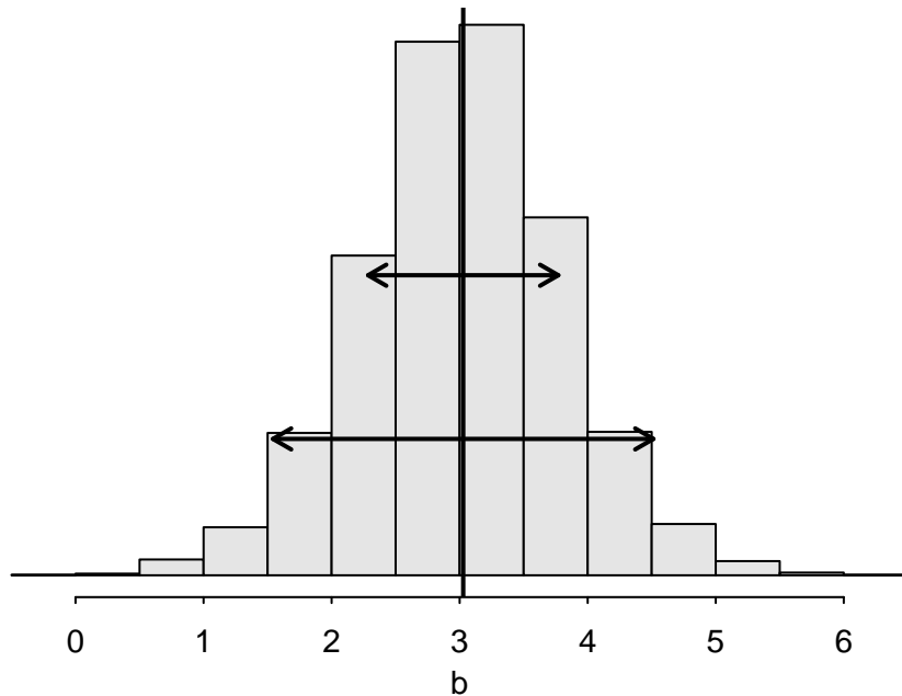
Posterior simulations of the slope, b , and posterior median \pm 1 and 2 std err
