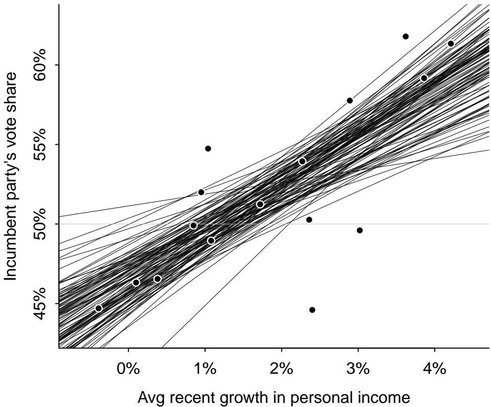
Data and 100 posterior draws of the line, y = a + bx
